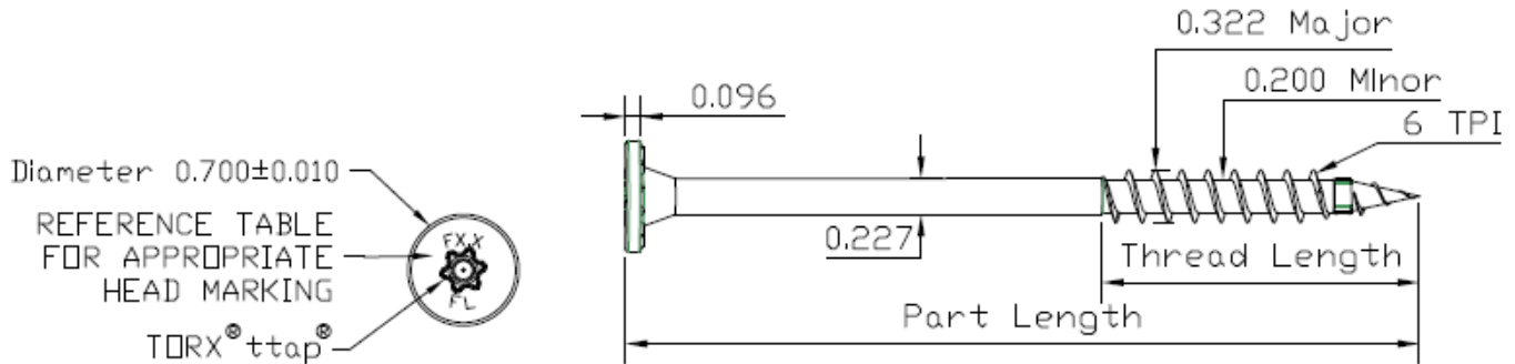
FIGURE 1. FASTENMASTER® FLATLOK®
