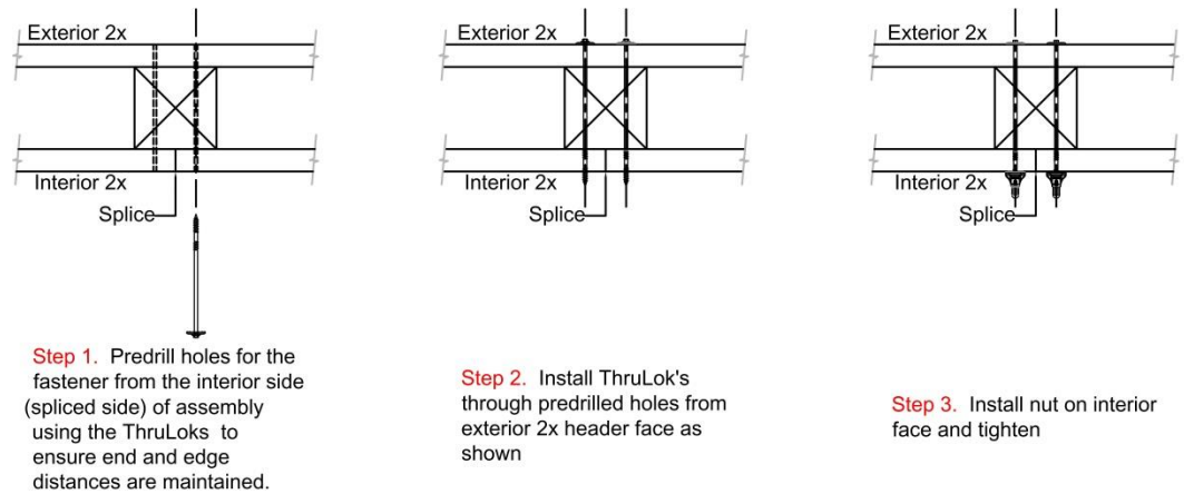
Figure 5b: Installation of Header with Splice on Interior Side of Column
