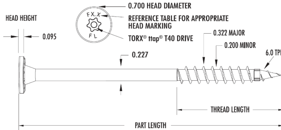
FIGURE 1: FastenMaster® FlatLOK®
