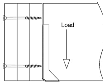
FIGURE 2b – Point Side Loading
