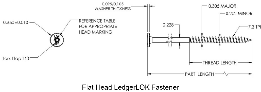
FIGURE 3—LEDGERLOK FASTENERS
